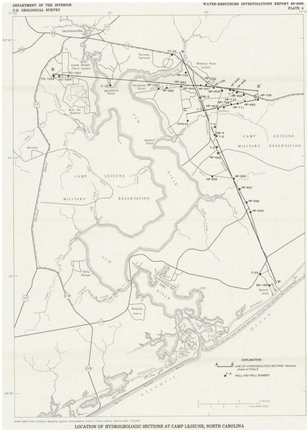
Exhibit I-2b. Base Area Geological Cross Sections 13
