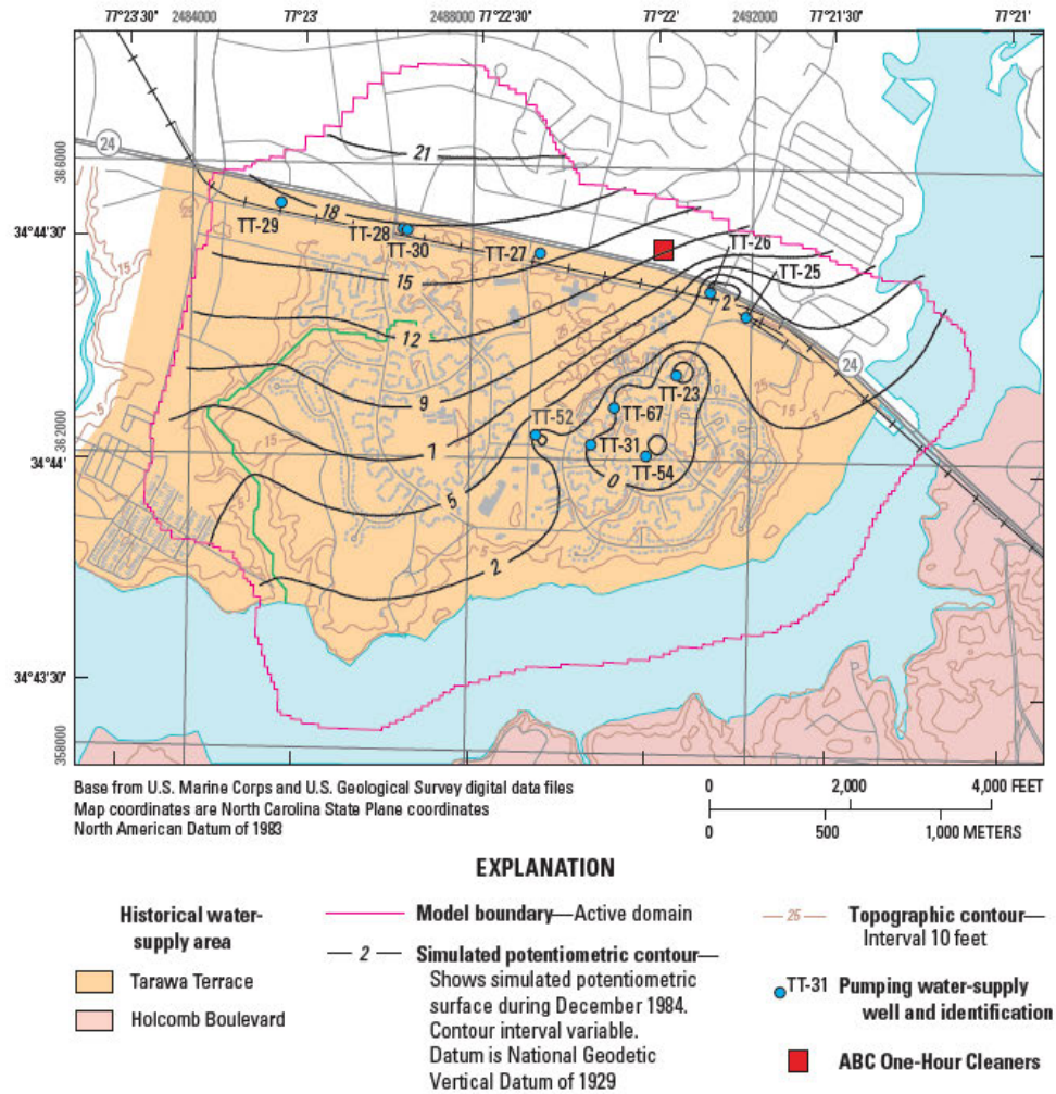
Figure C19. Simulated potentiometric levels, Upper Castle Hayne aquifer—Lower unit (model layer 3), stress period 408 (December 1984), Tarawa Terrace and vicinity, U.S. Marine Corps Base Camp Lejeune, North Carolina.
