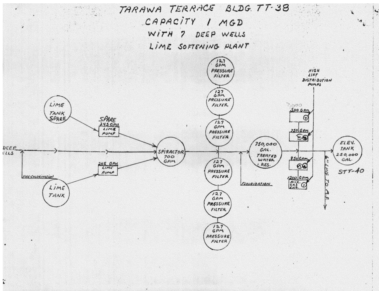
Exhibit I-4b. Schematic of TT-WTP [CLJA_WATERMODELING_07-0000003183]
