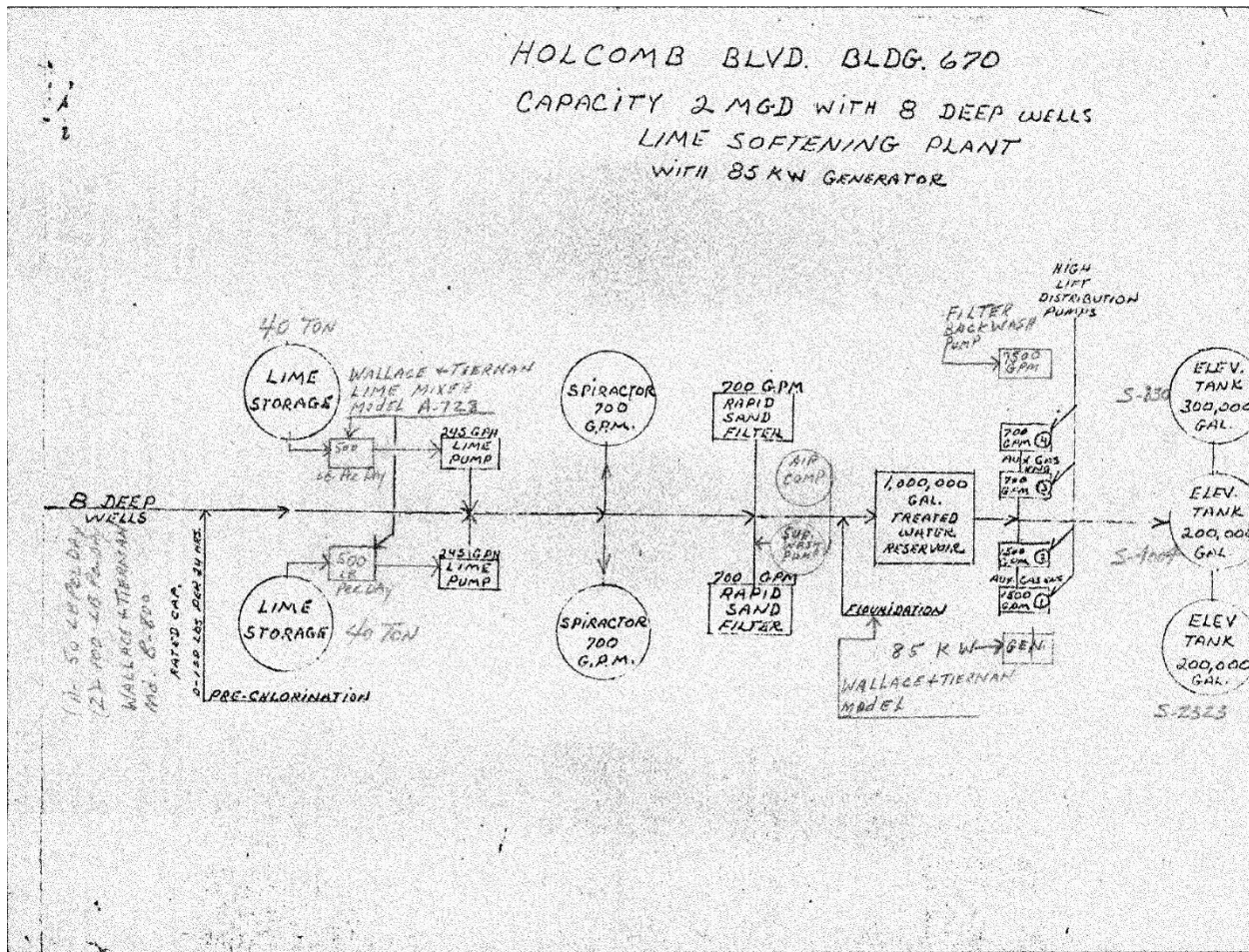
Exhibit I-4c. Schematic of HB-WTP [CLJA_WATERMODELING_07-0000003181] 14
