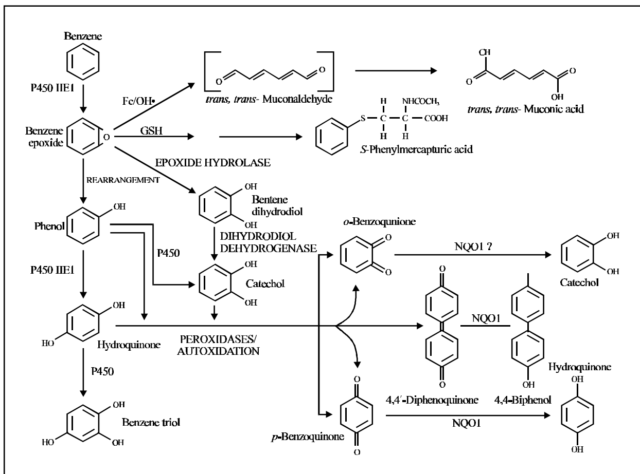
Figure 1. Major metabolic pathways in benzene toxicity.
