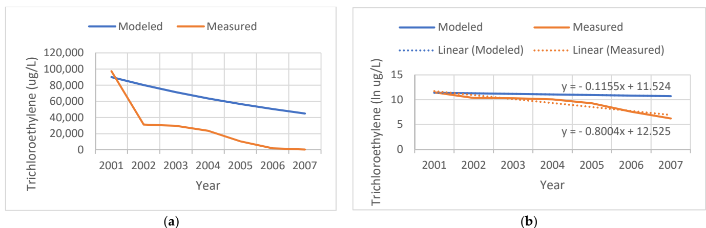
Figure 2. Comparison of the trichloroethylene (TCE) levels modeled (blue) versus measured (red) at a remediated site. (a) TCE levels in ug/L. (b) Natural log (ln) of TCE levels.
