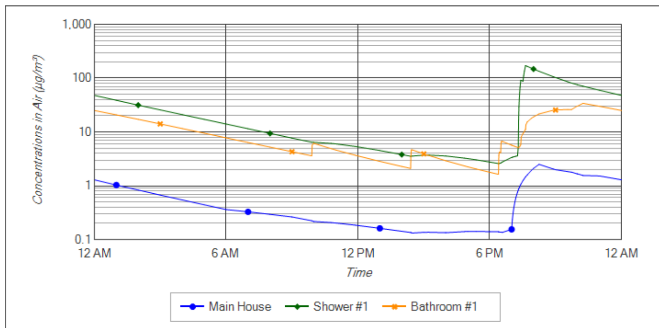
Figure 1. Calculated air concentrations in the shower, bathroom, and main house compartments for a 2-person household
