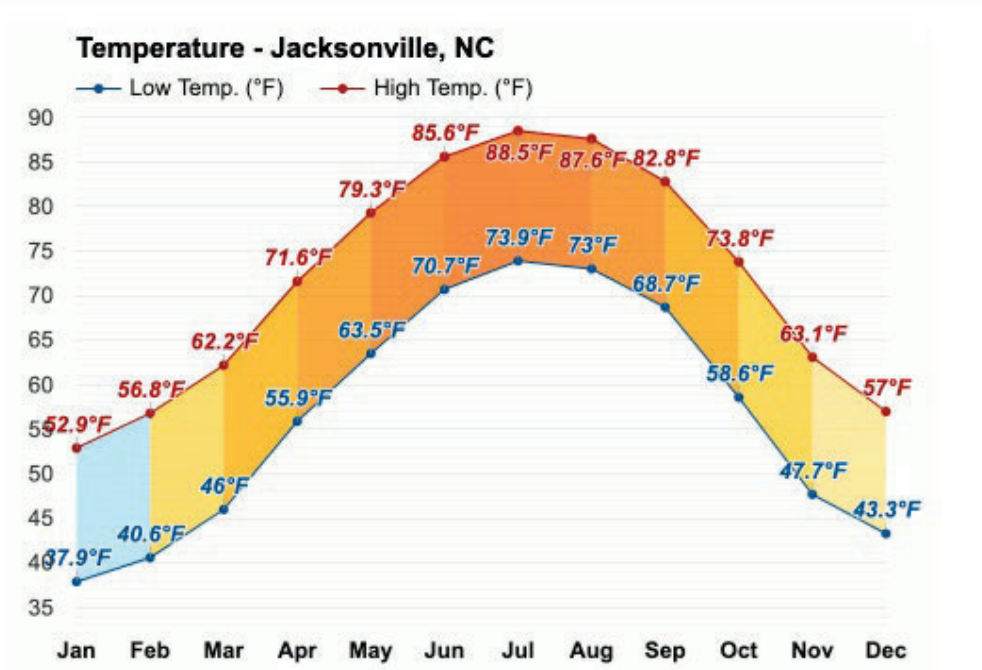
Figure 5. Average high and low monthly temperatures in Jacksonville, NC (reprinted from https://www.weather-us.com/en/north-carolina-usa/jacksonville-weather-march#google_vignette )
