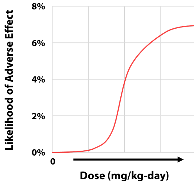
Figure 3.1 Dose-Response Curve
