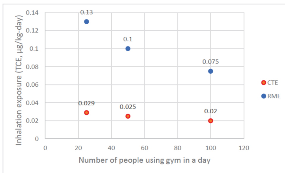
Figure 5. Relationship between the number of people using a gym facility in a day versus the CTE and RME inhalation exposure (SHOWER Model vs 4). The water concentration of TCE was set at 21.6 µg/L. Model default values were used for all other parameters.
