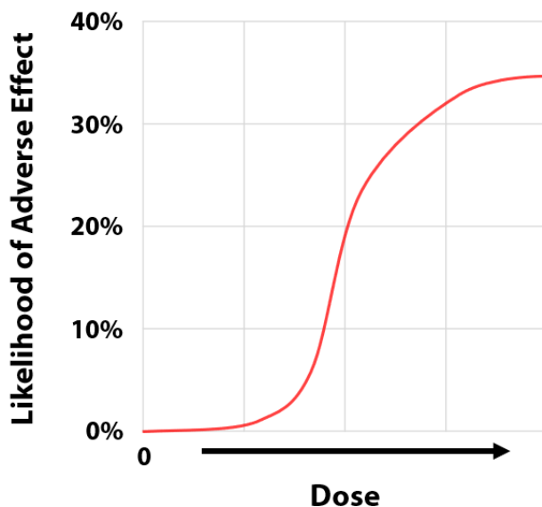
Figure 3.1 Dose-Response Curve
